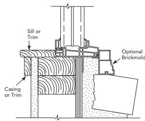
Sill Detail w/Optional Brickmold
